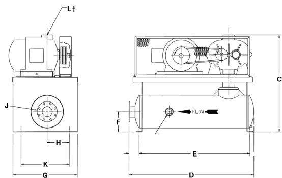
PneuPak "C" Package with discharge silencer
