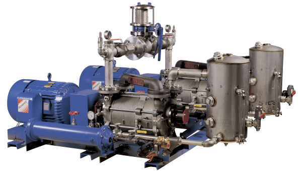
Optional all stainless steel package shown. Control panel not shown.
